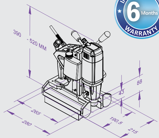
Technical Drawing
